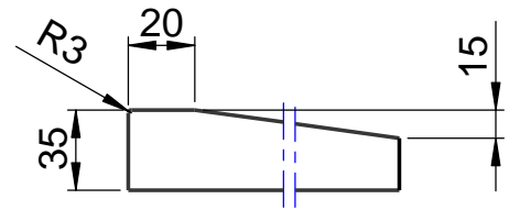
Detail Rand
