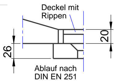
Detail Rand
